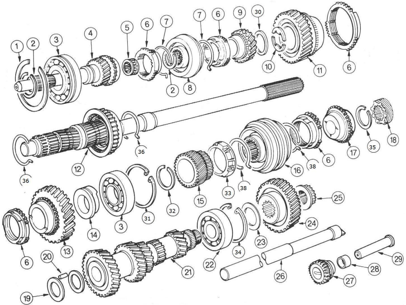
Ford Type 9 ( Type N) 5 speed gearbox parts list.
